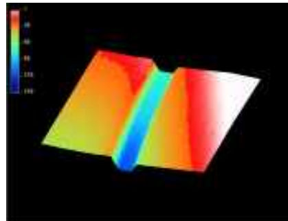
Rated breaking point on a beverage can
