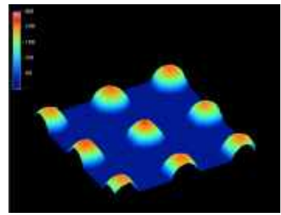
Ball Grid Array Topography
